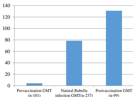
Figure 1: Geometric mean titer (GMT) of pre-vaccination, natural Rubella infection and post-vaccination sample.
